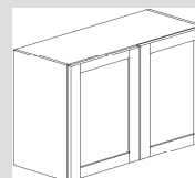
24H X 15D WALL 23-3/4"H X 15"D
