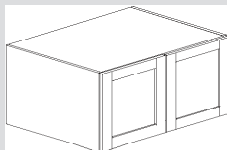
18H X 24D APPLIANCE WALL 17-5/8"H X 23-5/8"D
