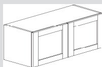
15H APPLIANCE WALL 15"H X 11 7/8"D
