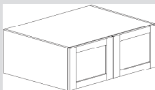
12H X 24D APPLIANCE WALL 11-3/4"H X 23-5/8"D
